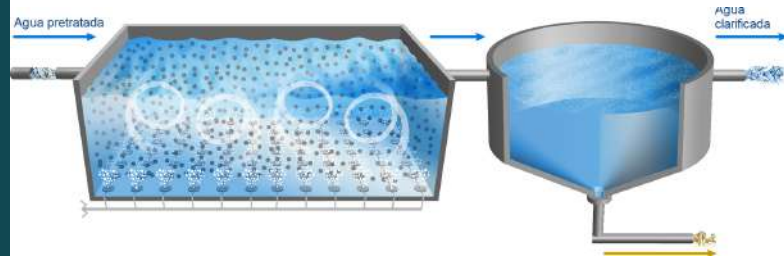
Moving Bed Bioreactor (MBBR)
