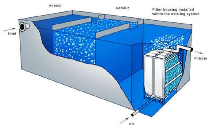
Membrane Bioreactor (MBR)
