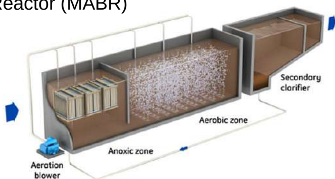
Membrane Aerated Biofilm Reactor (MABR)
